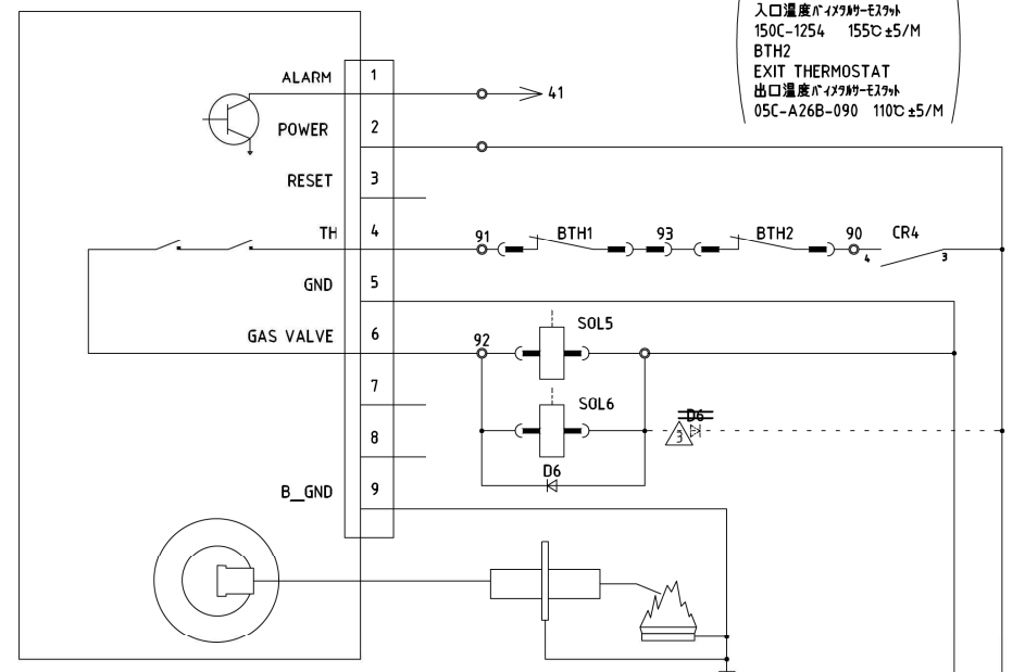
DIRECT SPARK IGNITION CONTROLS FENWAL 35-405200-001
