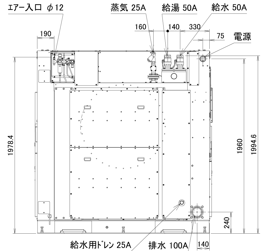
WN1180Z外観図
